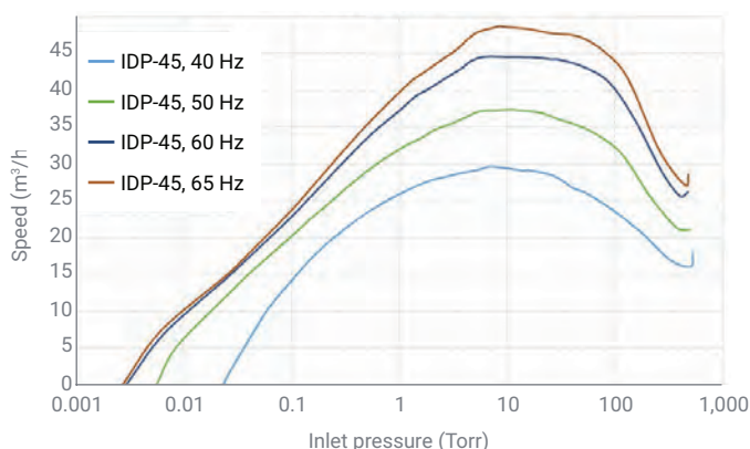
Figure 2. Agilent IDP-45 dry scroll pump pumping speed.
