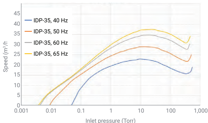
Figure 1. Agilent IDP-35 dry scroll pump pumping speed.
